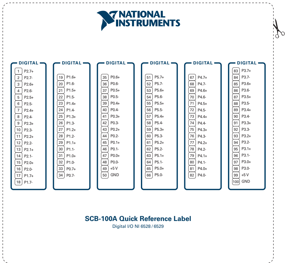
Figure 8. NI 6528/6529
