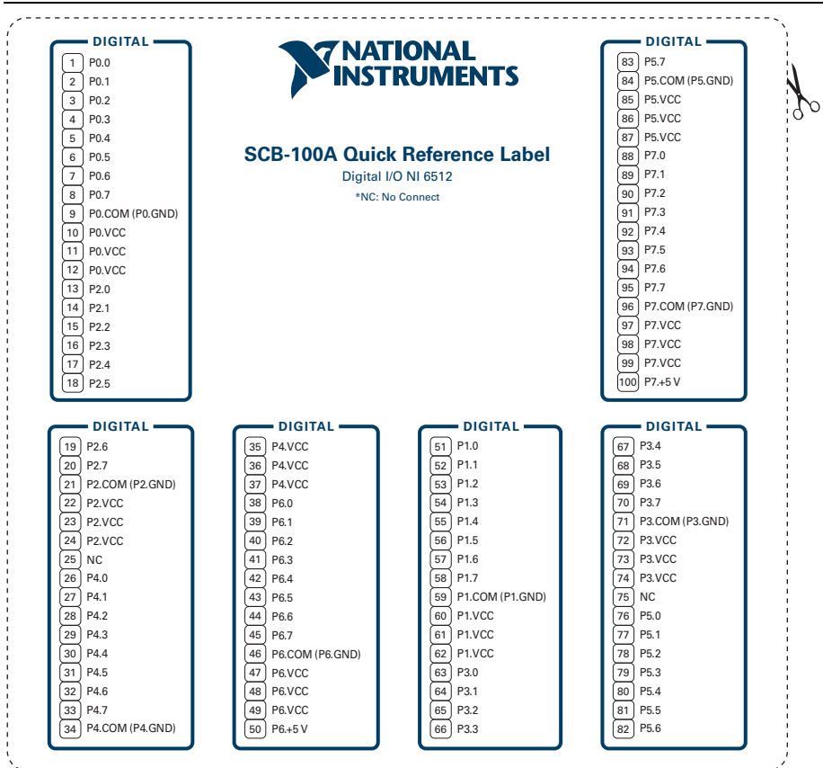
Figure 4. NI 6512
