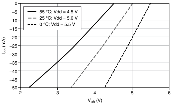
Figure 4. DIO (P0.<0..7>): I oh versus V oh
