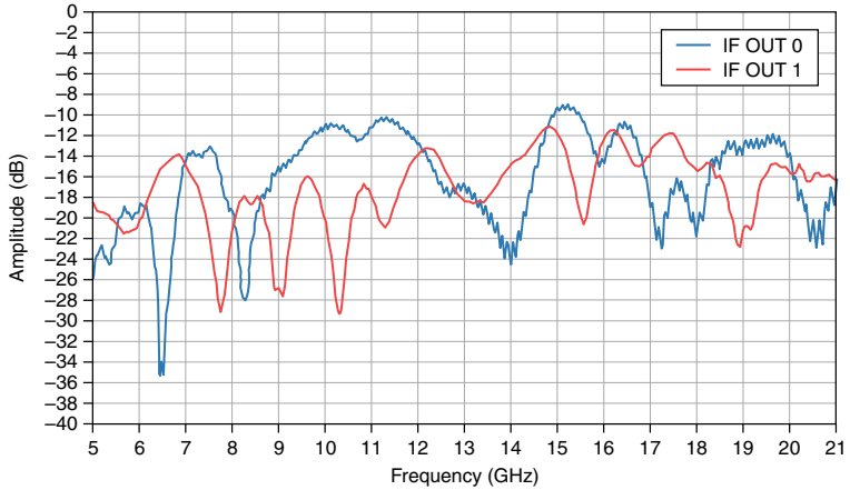
Figure 36. PXle-3622 IF OUT Port Return Loss, Measured
