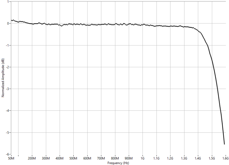
Figure 11. Analog Output Dual Channel Mode Frequency Response, Measured 16
