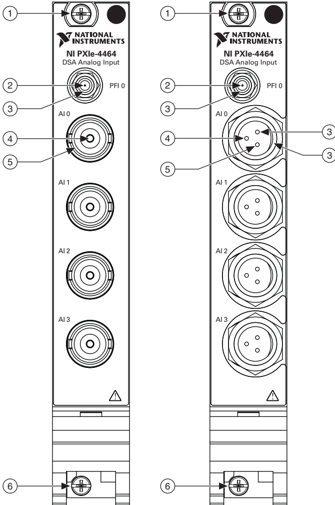
Figure 1. NI PXIe-4464 BNC and mXLR Connector Front Panel
