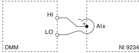
Figure 5. IEPE Current Verification Connections to the NI 9234
