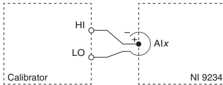
Figure 1. Accuracy Verification Connections to the NI 9234
