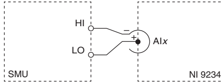
Figure 7. IEPE Compliance Voltage Verification Connections to the NI 9234 (IEPE Source Compliance Voltage Measurement)
