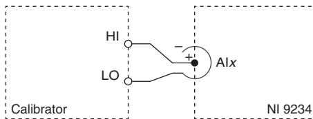
Figure 2. Gain Matching Verification Connections to the NI 9234
