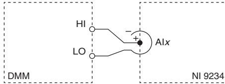
Figure 6. IEPE Compliance Voltage Verification Connections to the NI 9234 (IEPE Source Short Circuit Current Measurement)
