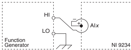
Figure 4. CMRR Verification Connections to the NI 9234
