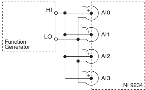
Figure 3. Phase Matching Verification Connections to the NI 9234
