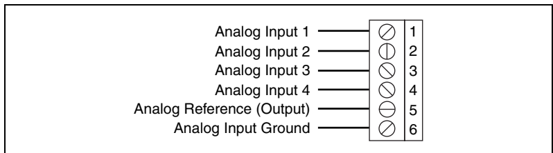
Figure 13. Analog Input Terminal Block Pin Assignment
