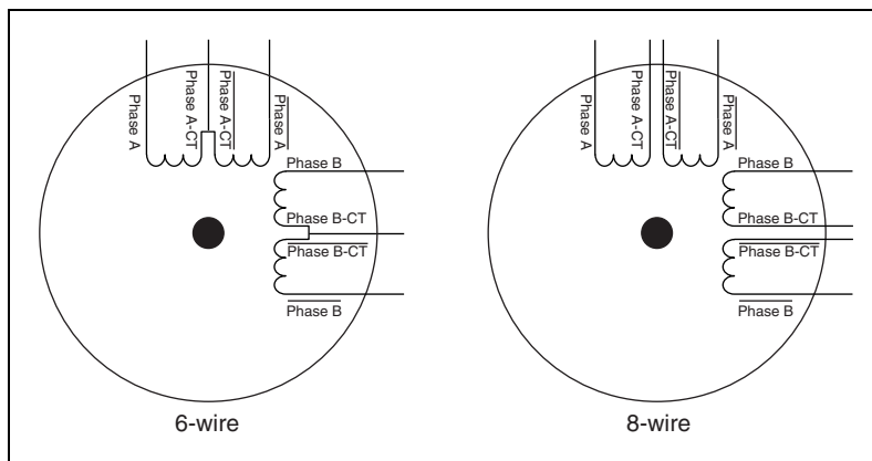
Figure 17. 6-Wire and 8-Wire Stepper Motors
