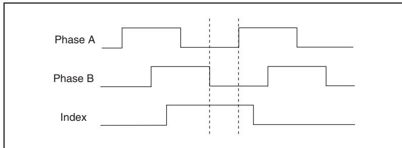
Figure 7. Encoder Signal Phasing, CW Rotation
