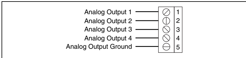
Figure 14. Analog Output Terminal Block Pin Assignment
