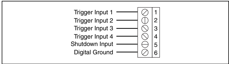
Figure 11. Trigger Terminal Block Pin Assignment
