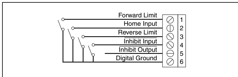
Figure 10. Limit Switch Terminal Block Pin Assignment (Passive Limit Switch Connection Example)
