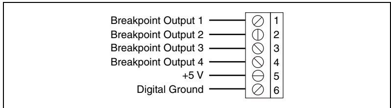
Figure 12. Breakpoint Terminal Block Pin Assignment
