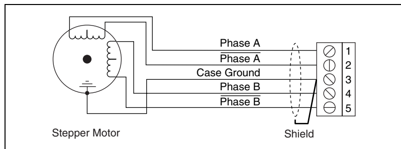
Figure 4. Typical Full-Coil Stepper Motor (2-Phase Type) Terminal Block Pin Assignment
