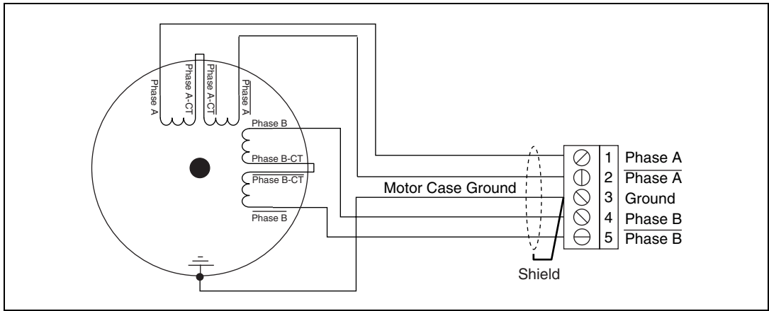
Figure 18. Series Stepper Motor Wiring (Higher Torque, Lower Speed)
