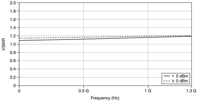
Figure 6. Measured VSWR
