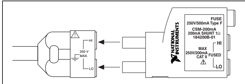
Figure 1. Connecting the CSM to the P4-BJ2 Cable Included with the NI 4050
