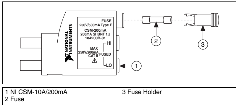
Figure 7. Removing the Fuse
