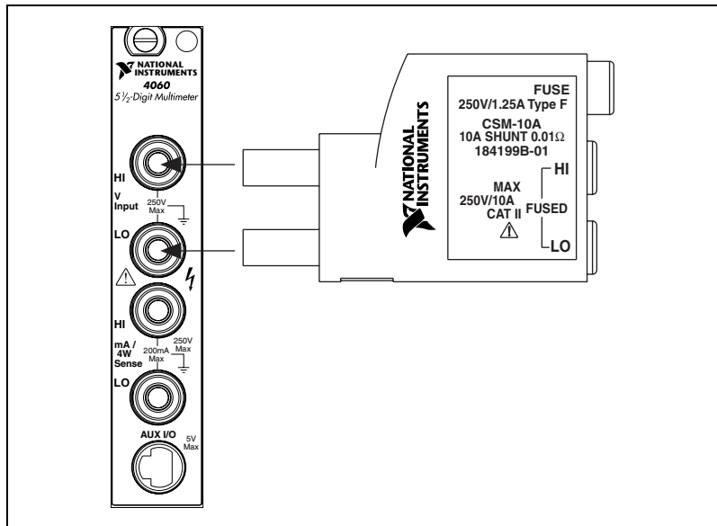
Figure 2. Connecting the CSM to the NI 4060
