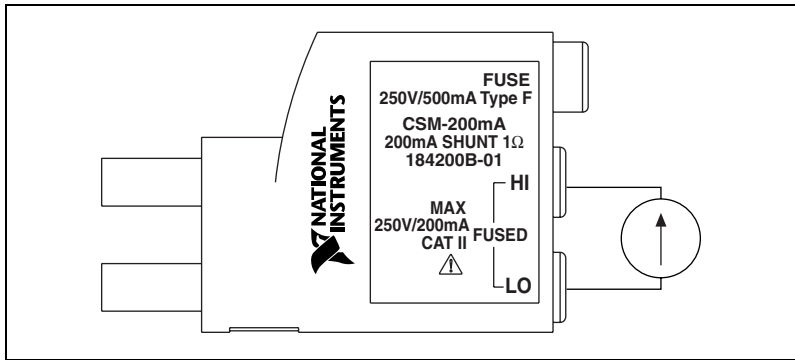
Figure 4. Connecting Current to the CSM
