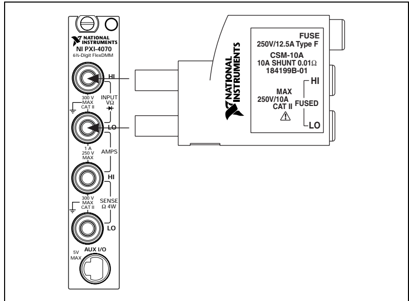
Figure 3. Connecting the CSM to the NI 4070
