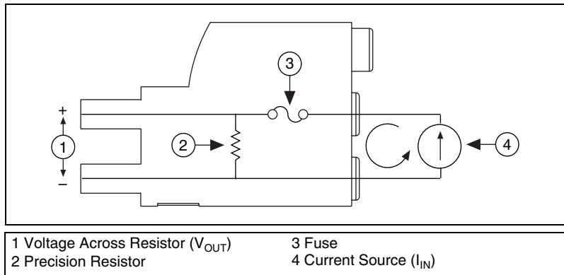
Figure 5. CSM Internal Construction
