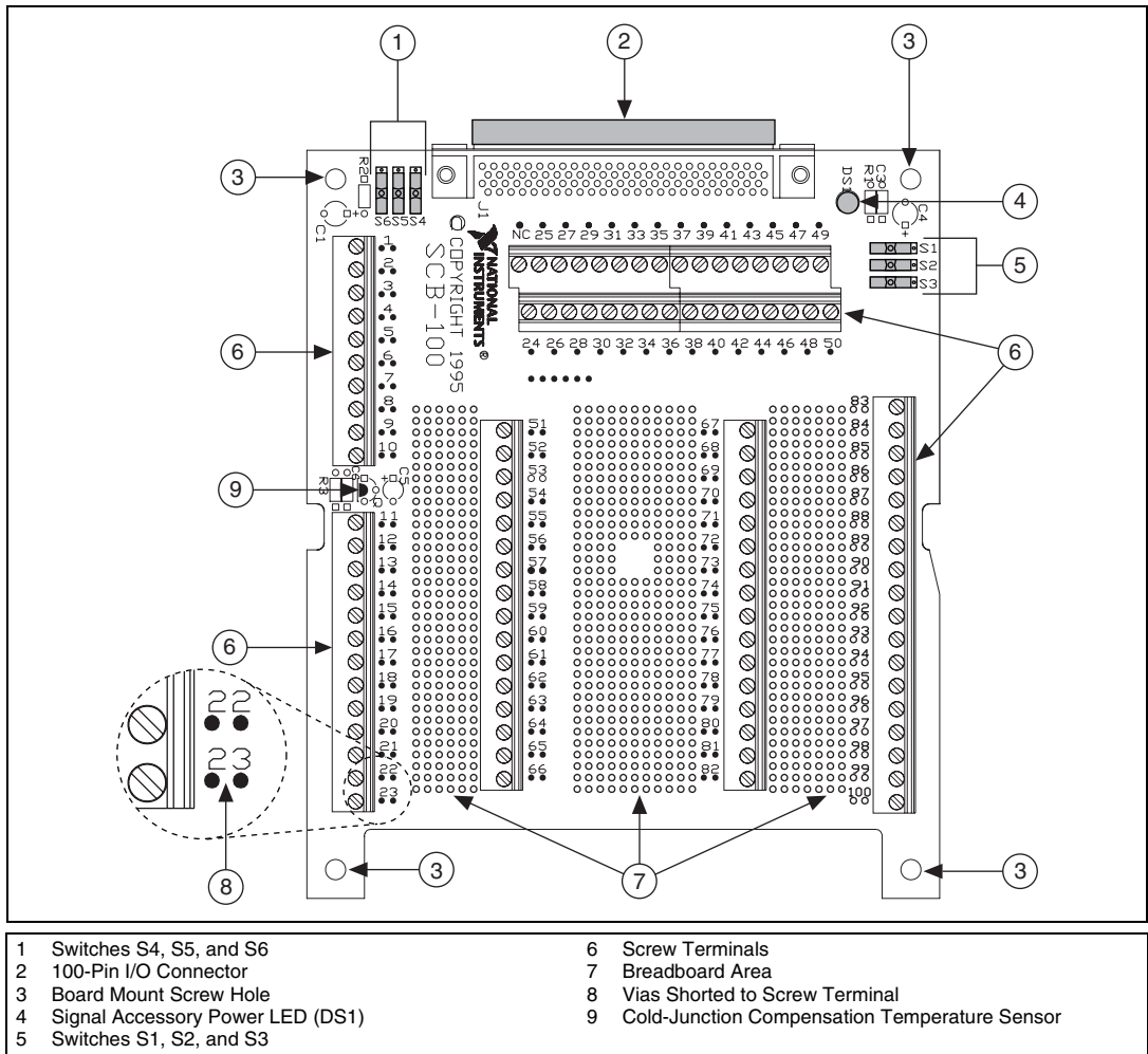
Figure 2. SCB-100 Board Parts Locator Diagram
