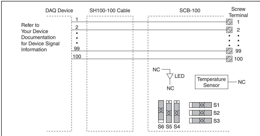
Figure 3. DIO/Passthrough Mode Switch Setting
