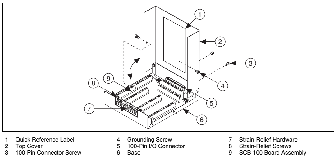
Figure 1. SCB-100 Connector Block
