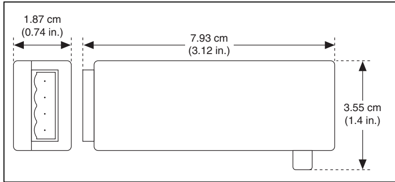
Figure 4. SCC-AI Dimensions
