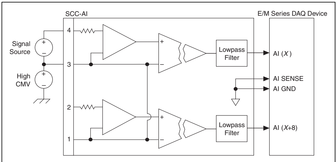
Figure 3. Ground-Referenced Signal Connection for the SCC-AI with High Common-Mode Voltage (One Channel)
