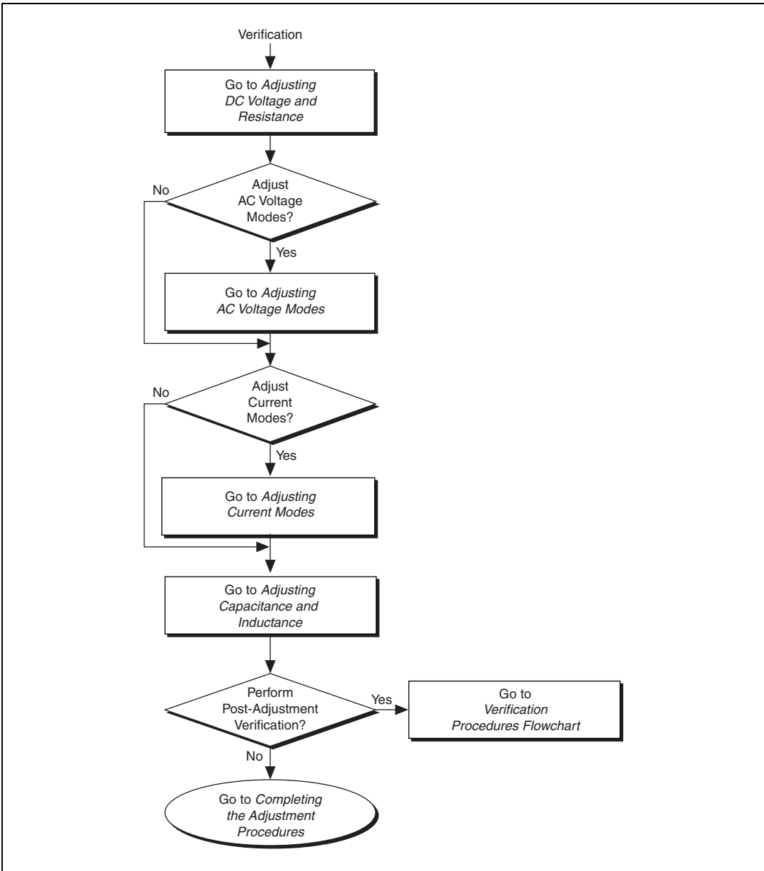
Figure 2. Adjustment Procedures Flowchart
