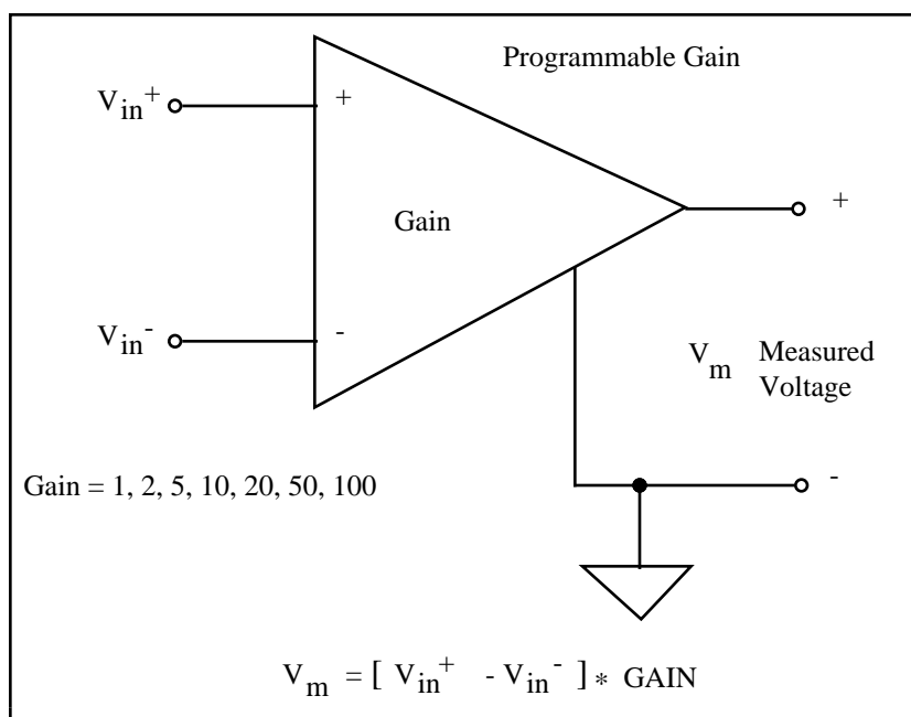
Figure 2-6. AT-MIO-16X PGIA
