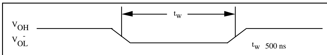
Figure 2-13. EXTSTROBE* Signal Timing
