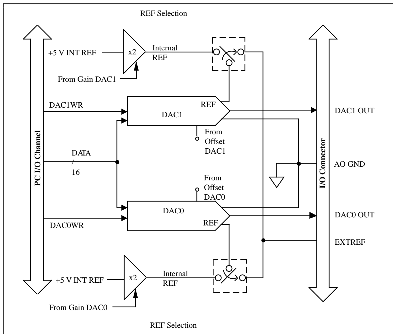
Figure 3-9. Analog Output Circuitry Block Diagram
