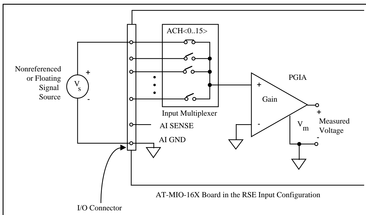
Figure 2-9. Single-Ended Input Connections for Nonreferenced or Floating Signals
