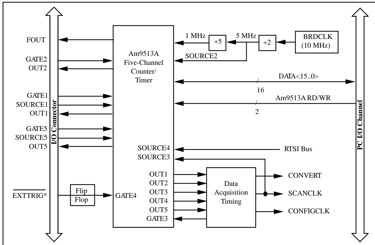
Figure 3-17. Timing I/O Circuitry Block Diagram
