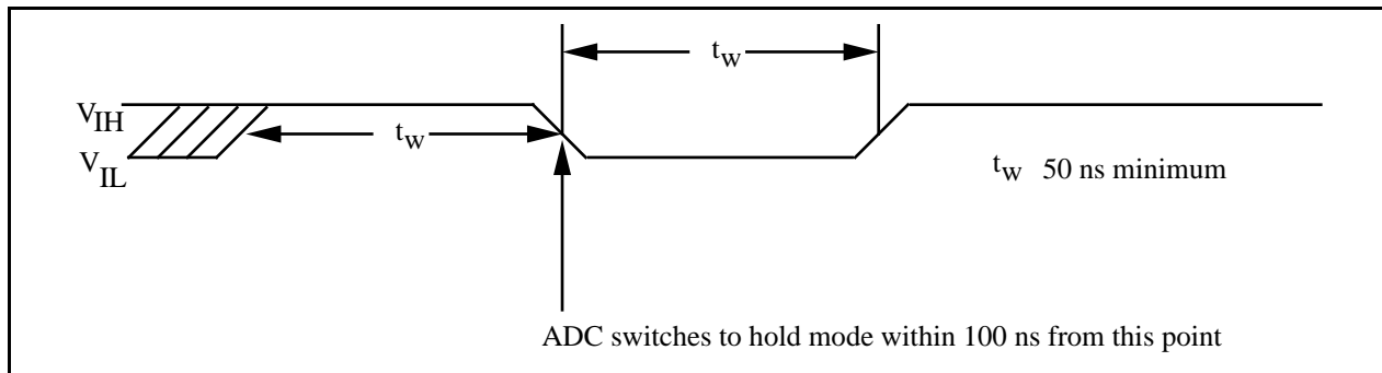
Figure 2-14. EXTCNV* Signal Timing
