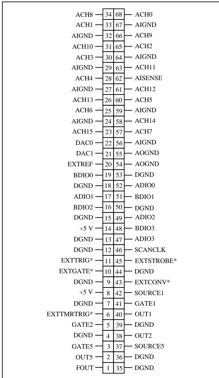
Figure 2-5. AT-MIO-16X 68-Pin I/O Connector
