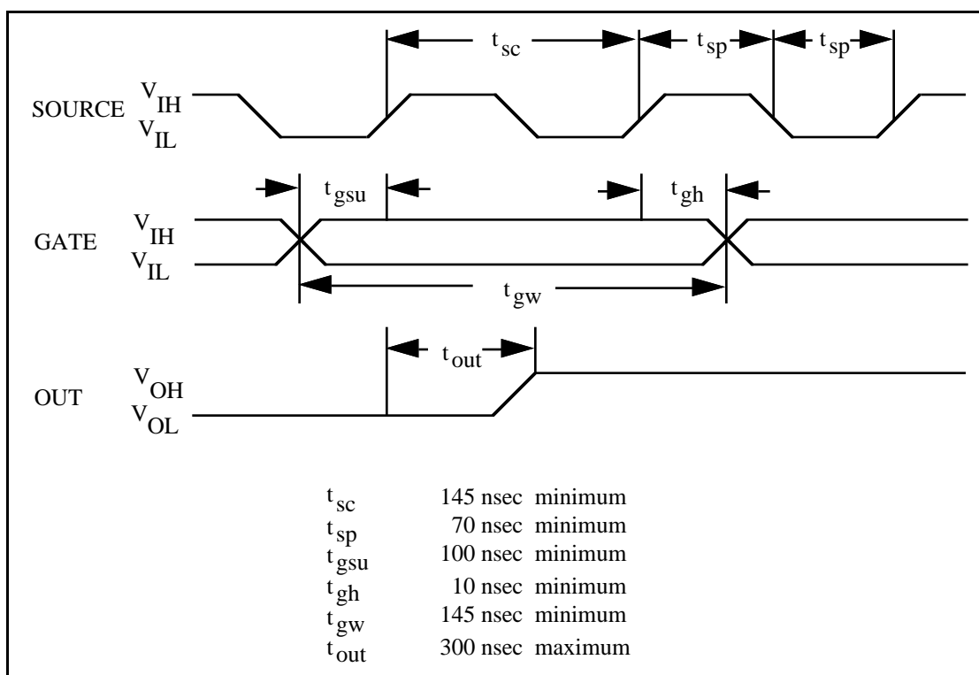
Figure 2-19. General-Purpose Timing Signals
