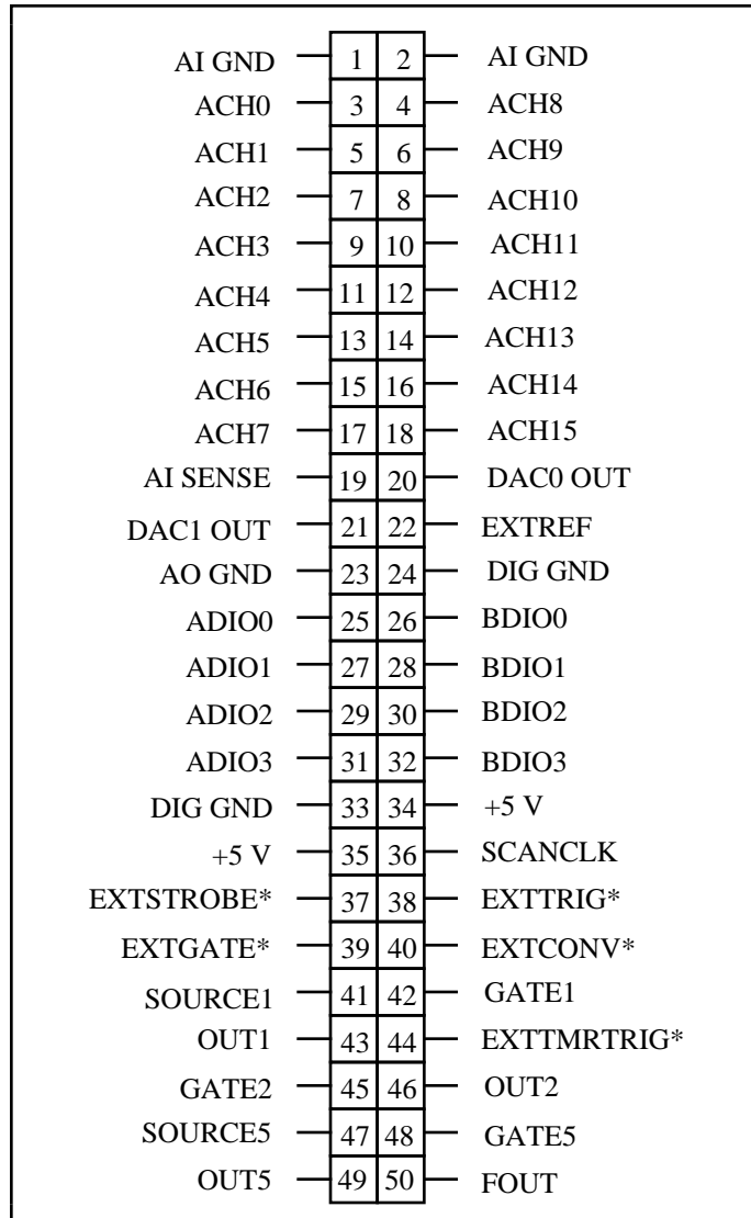
Figure 2-4. AT-MIO-16X 50-Pin I/O Connector
