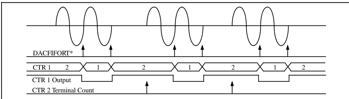
Figure 3-15. FIFO Pulsed Waveform Generation Timing
