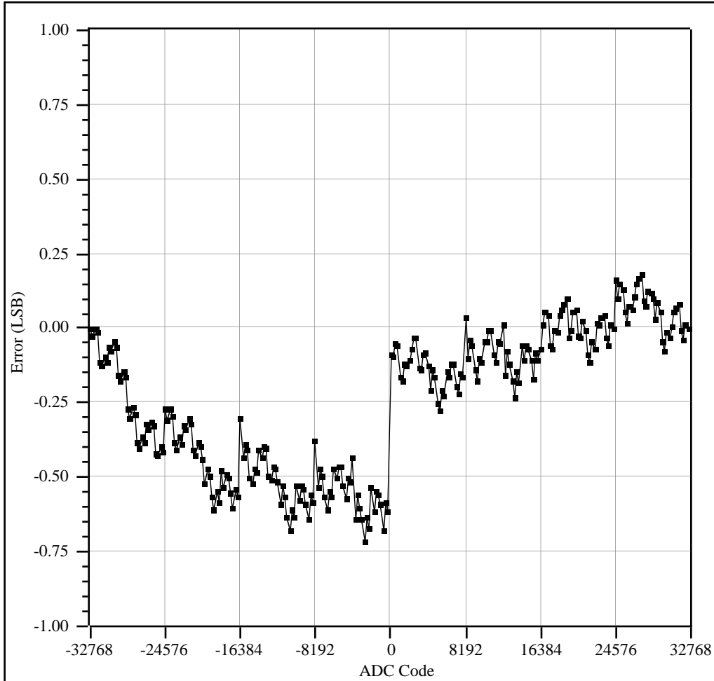
Figure A-1. Typical Relative Accuracy of Analog Input Circuitry
