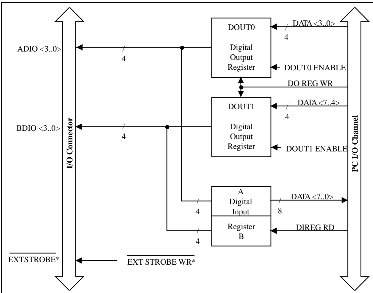
Figure 3-16. Digital I/O Circuitry Block Diagram
