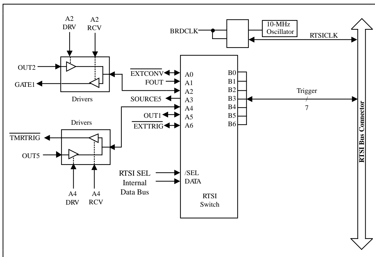
Figure 3-19. RTSI Bus Interface Circuitry Block Diagram
