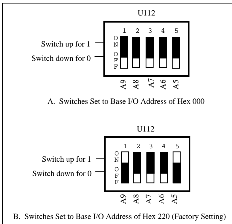
Figure 2-3. Example Base I/O Address Switch Settings
