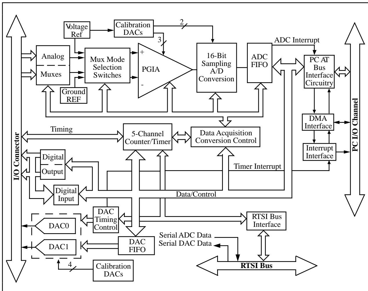
Figure 3-1. AT-MIO-16X Block Diagram
