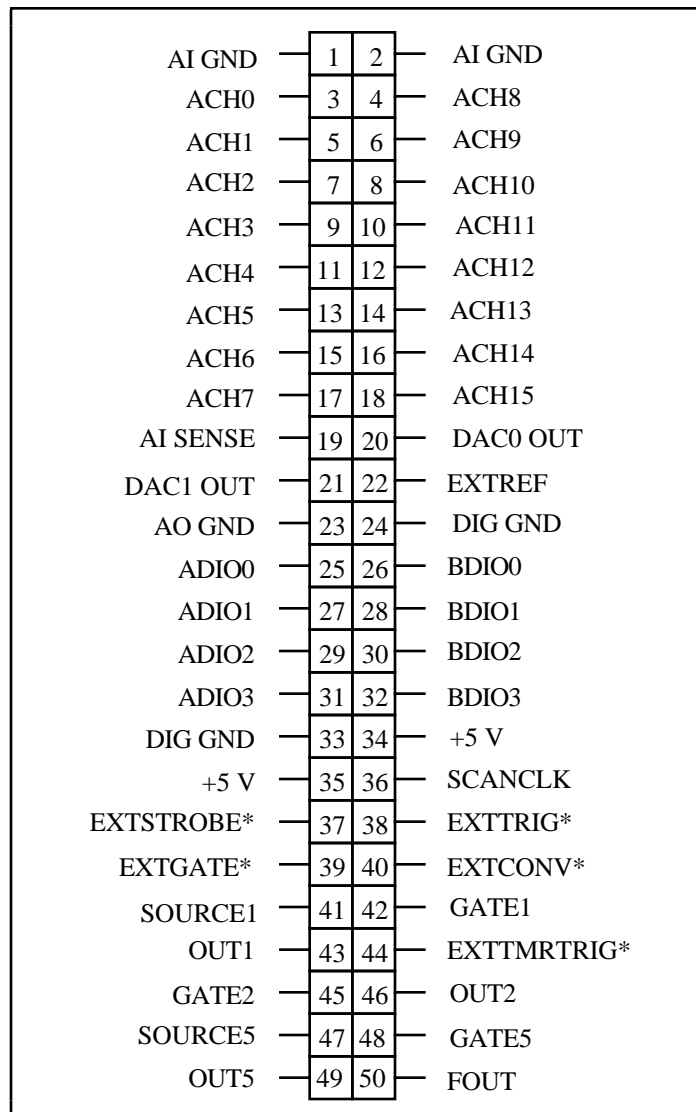
Figure B-1. AT-MIO-16X 50-Pin I/O Connector
