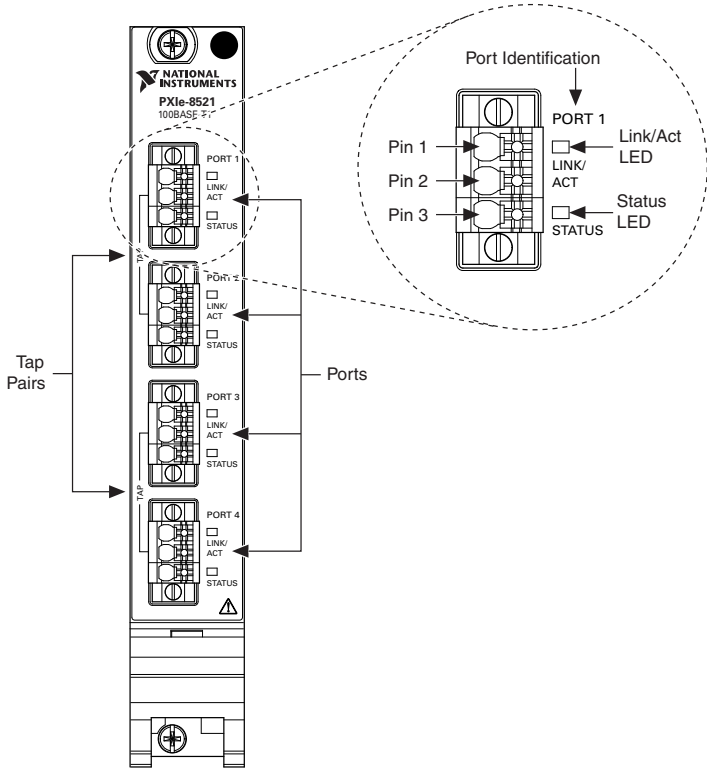
Figure 3. PXle-8521 Pinout
