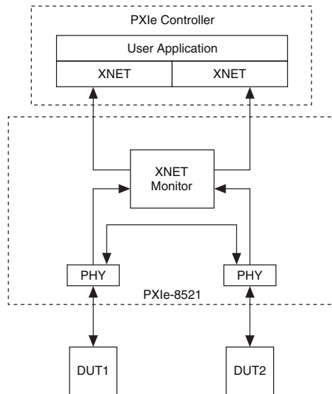
Figure 6. Tap Mode
