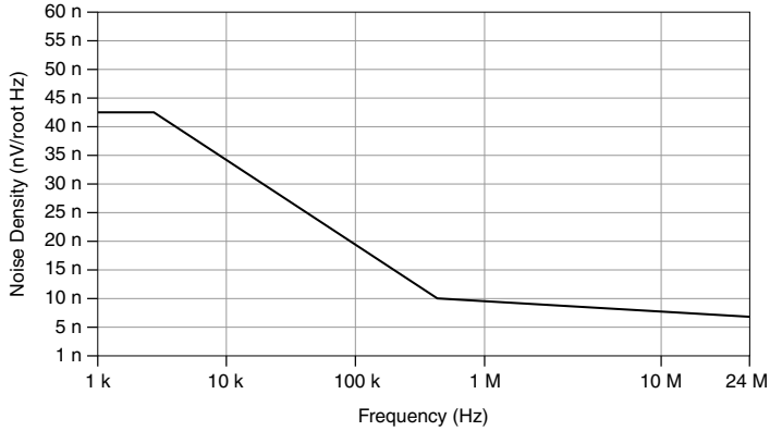
Figure 4. PXI-5122 Spectral Noise Density, 0.2 V Input Range, Noise Filter Enabled, 1 M \Omega Input Impedance, Nominal
