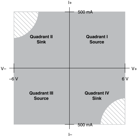
Figure 1. PXle-4145 Quadrant Diagram, All Channels
