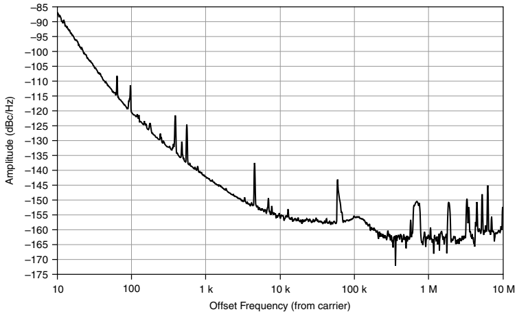
Figure 13. Internal Sample Clock Phase Noise
