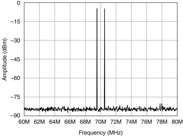
Figure 10. Measured Analog Output Two-Tone IMD
