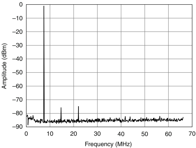
Figure 9. Measured Analog Output Single-Tone Distortion (Carrier Frequency = 7.36 MHz, Inverse Sync Filter OFF, Output Amplitude = -3 dBFS)
