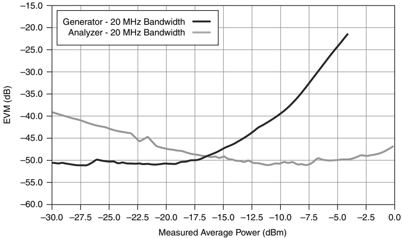
Figure 30. 802.11a/g RMS EVM Versus Measured Average Power 17 , 5,810 MHz, Channel Tracking Enabled, Typical
