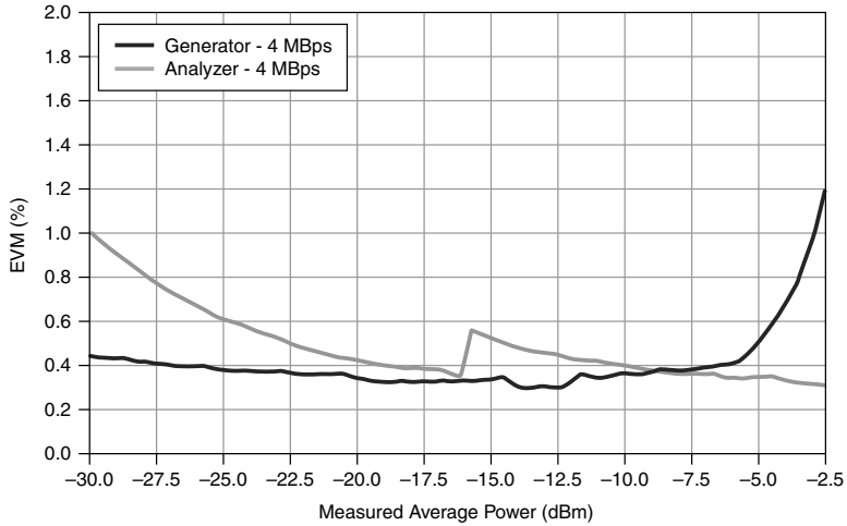
Figure 31. 802.11b RMS EVM Versus Measured Average Power 19 , Typical
