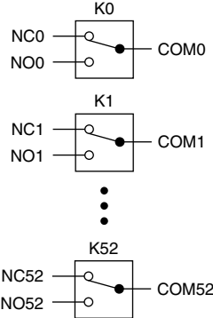
Figure 1. NI PXI-2522 Power-On State
