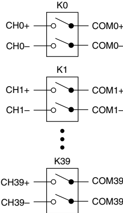
Figure 1. NI PXI-2521 Power-On State
