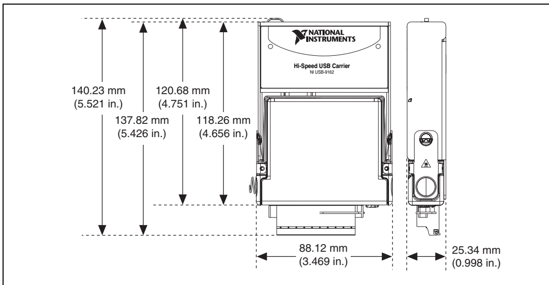
Figure 2. NI USB-9481 Device in Millimeters (Inches)
