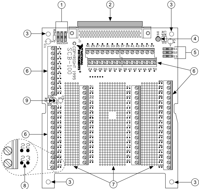
Figure 2. SCB-100 Board Parts Locator Diagram
