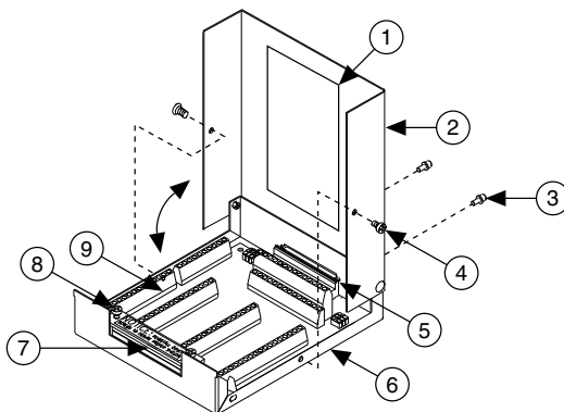
Figure 1. SCB-100 Parts Locator Diagram
