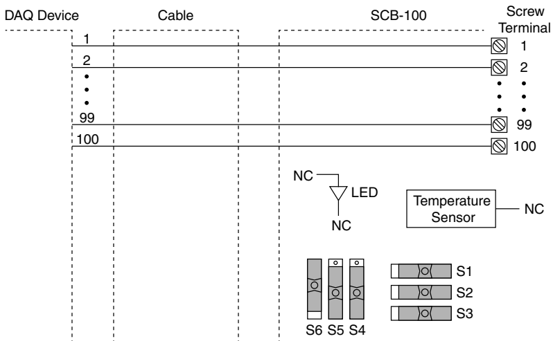
Figure 3. Direct Feedthrough Mode Switch Setting
