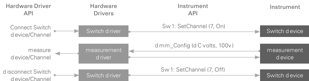
FIG 18 Example of hardware driver APIs for a signal input
