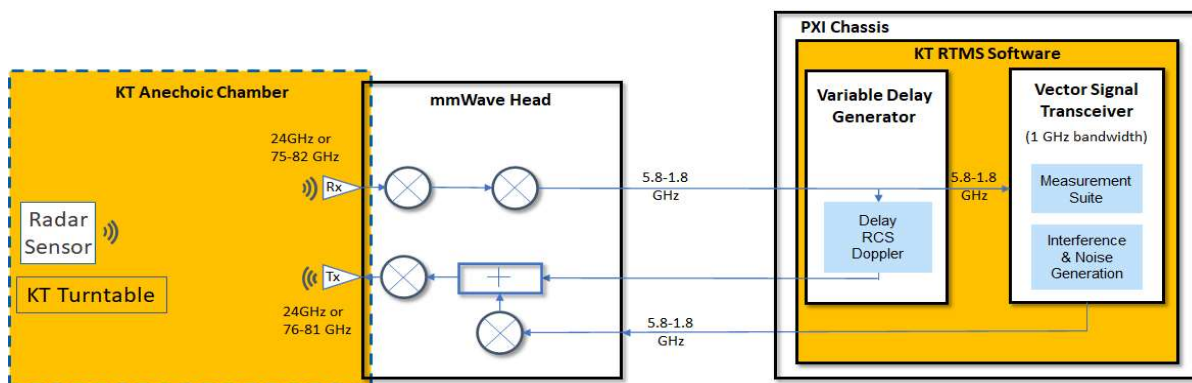
Figure 1. KT VRTS Solution System diagram
