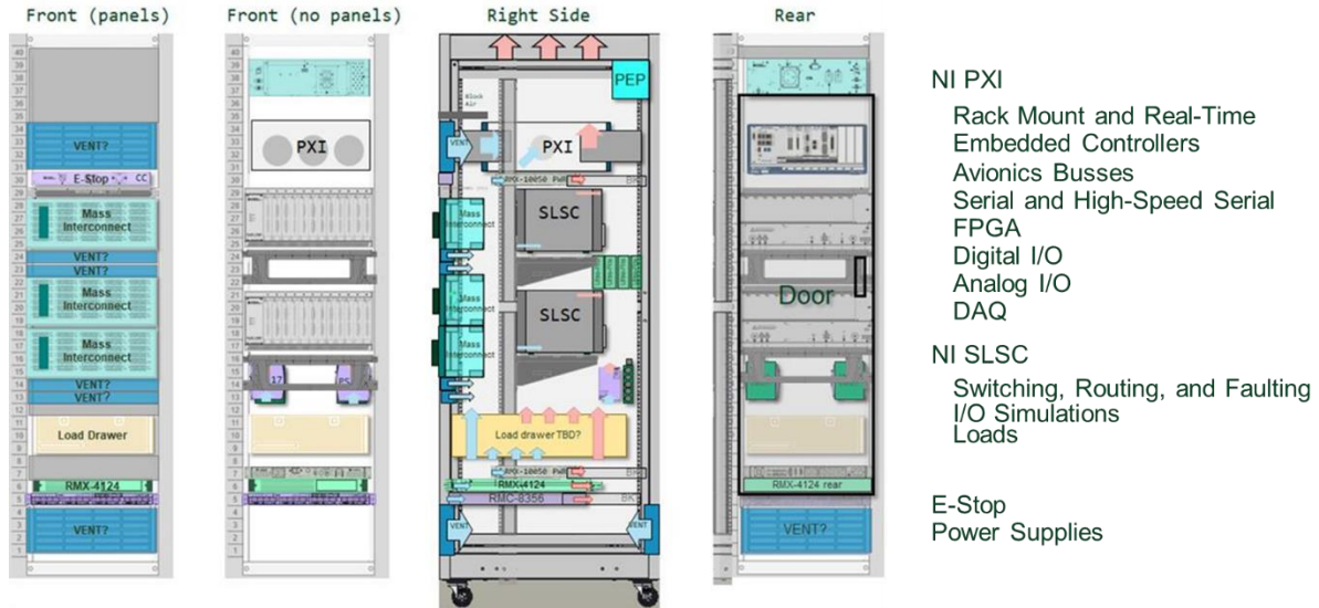
Figure 13. Conceptual LRU HIL Test Rack
