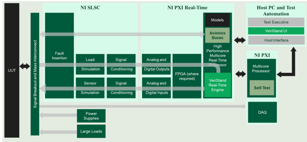
Figure 10. Signal-Flow Architecture of a Modular and Flexible HIL Test System
