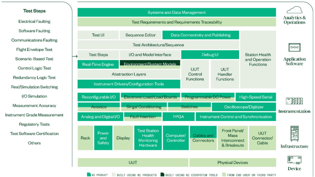
Figure 1. Key Hardware and Software Components of a Hardware-in-the-Loop Test System
