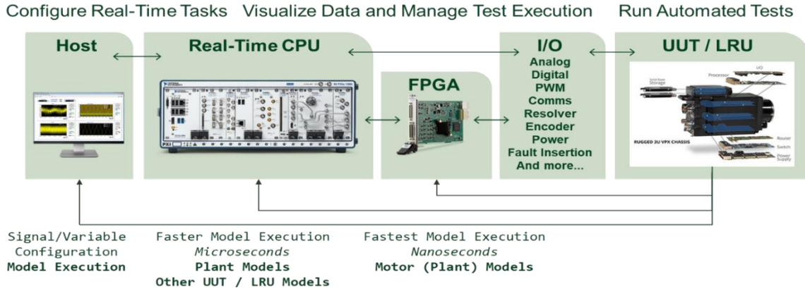
Figure 12. VeriStand Coordinates and Deploys Models across Different Processors
