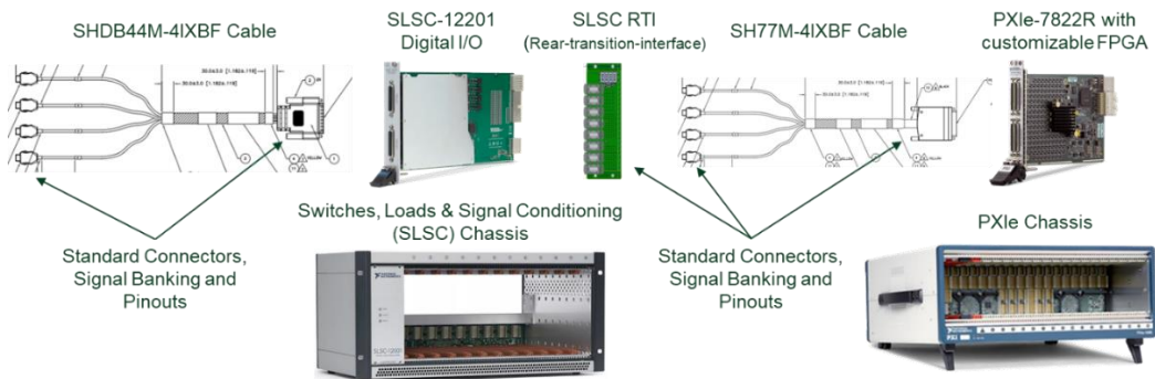
Figure 8. Example Digital IO Signal Path
