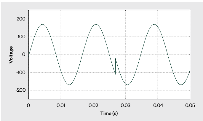
FIGURE 4 Simulating Phase Jump
