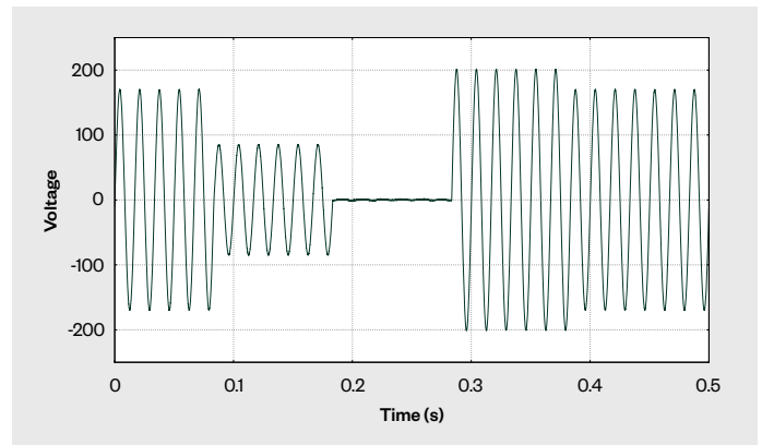
FIGURE 5 Simulating abnormal voltages (sags, swells, and drop outs)
