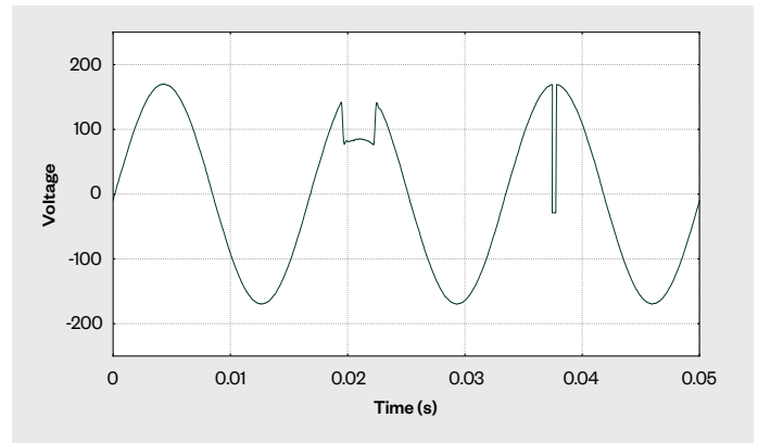
FIGURE 3 Simulating Sub-cycle Transients
