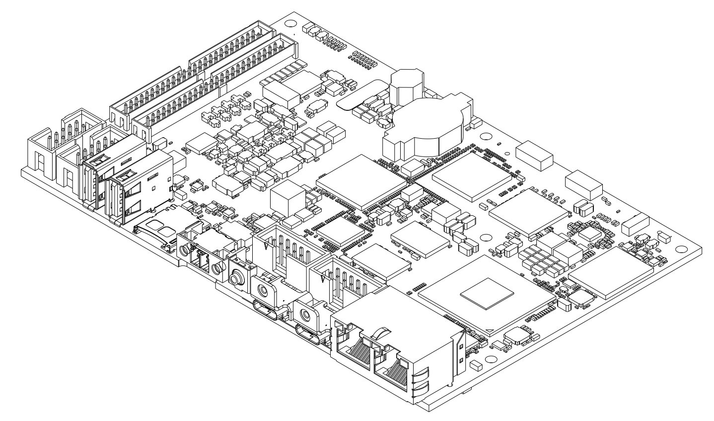
ISOMETRIC VIEW
