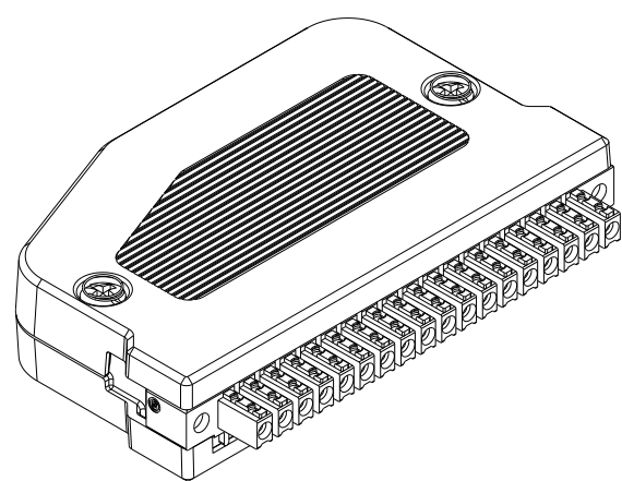
ISOMETRIC VIEW WITH 18POS CONNECTOR
