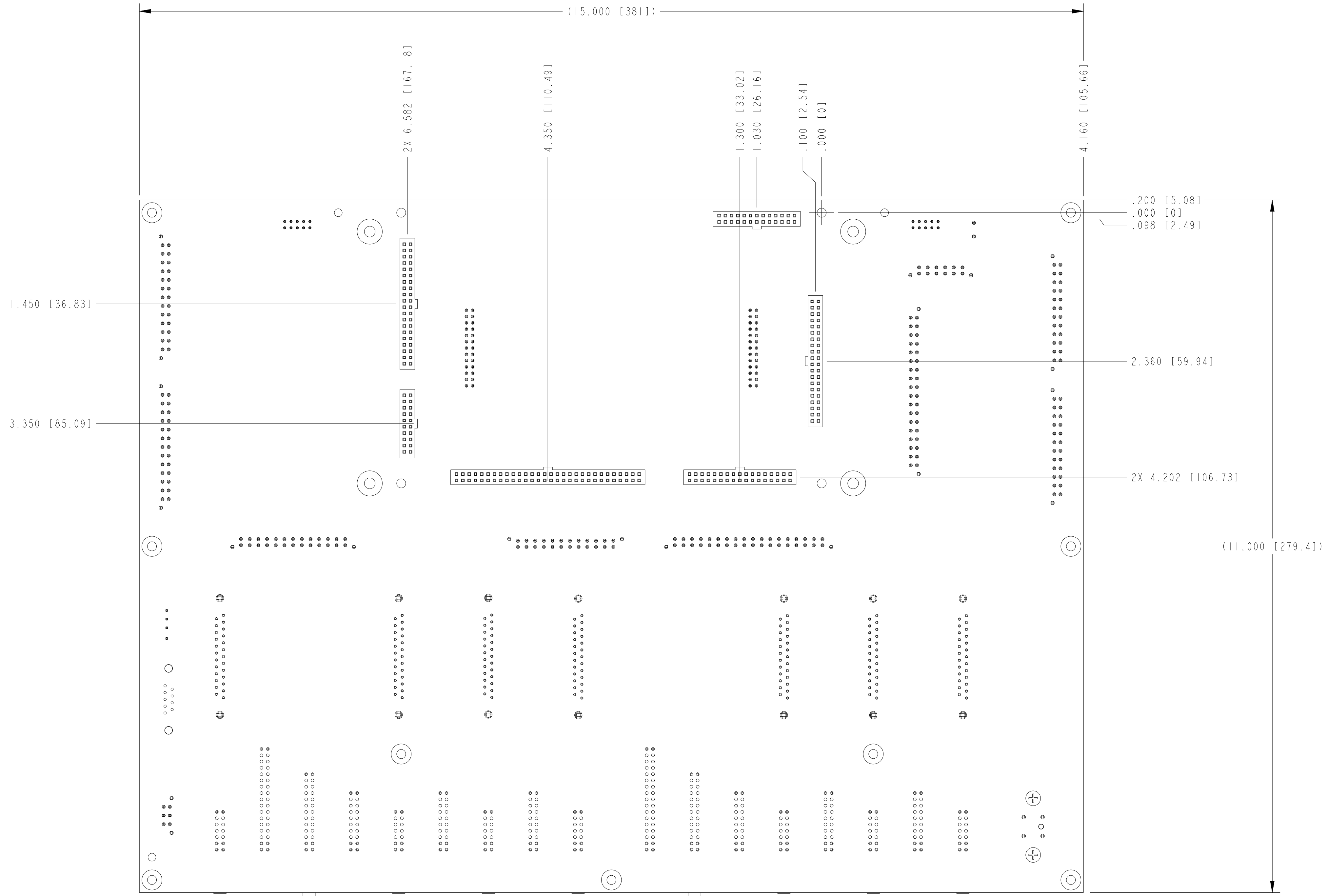
BOTTOM VIEW
