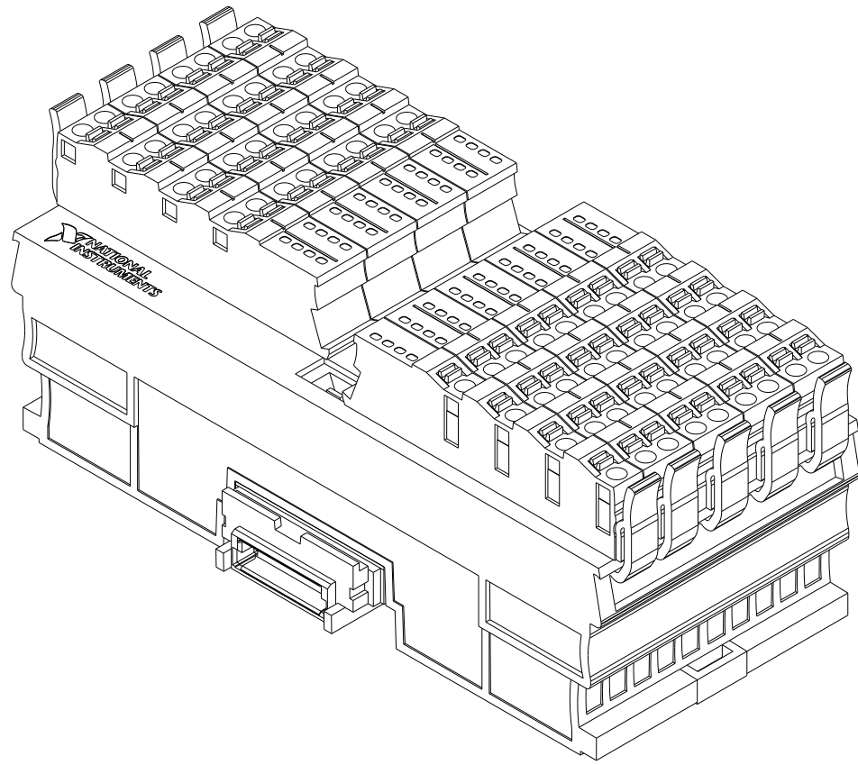
ISOMETRIC VIEW
