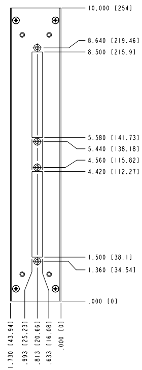
CA-1000, DIMENSIONED CUSTOMER DRAWING 777664-01
