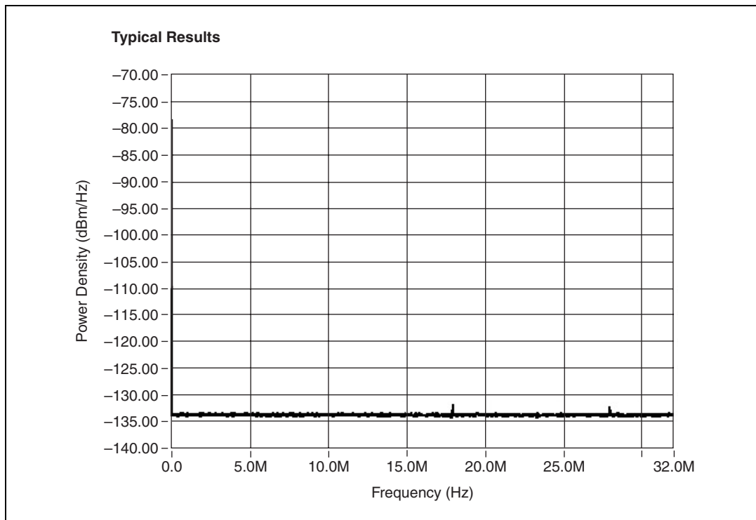
Figure 1. Noise Density (Dither Disabled, Input Terminated)
