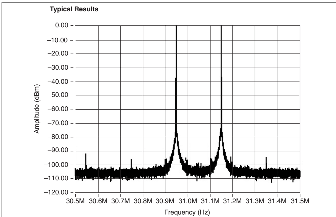
Figure 2. Intermodulation Distortion
