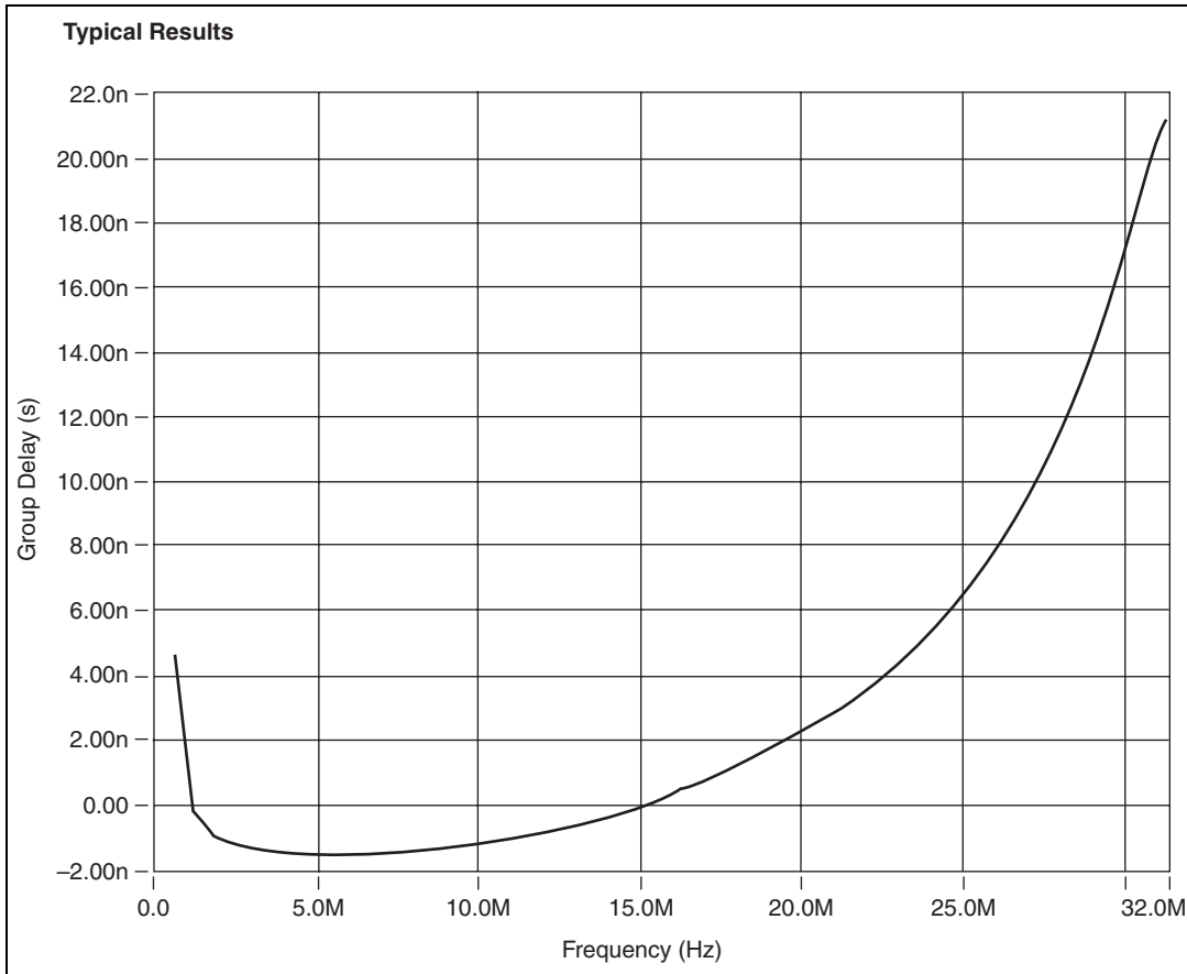
Figure 4. Group Delay versus Frequency
