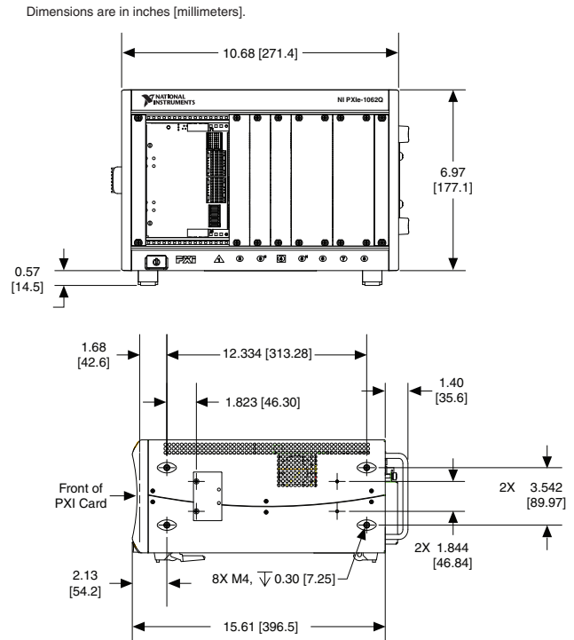
Figure 3. NI PXIe-1062Q Dimensional Drawings
