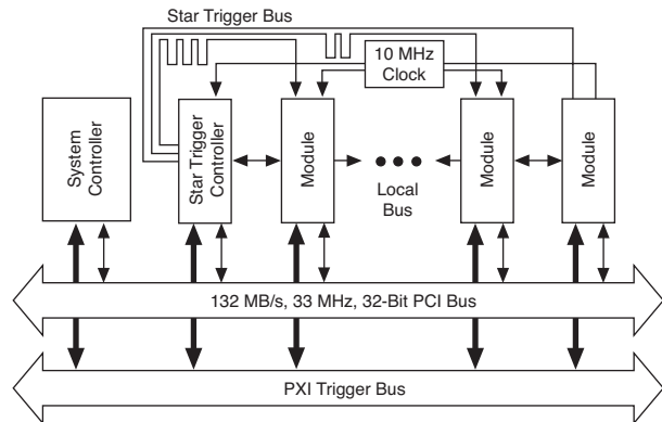
Figure 3. Diagram of Synchronization Features in the PXI Backplane
