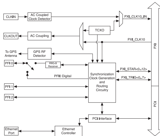
Figure 2. Functional Overview of the PXI-6682
