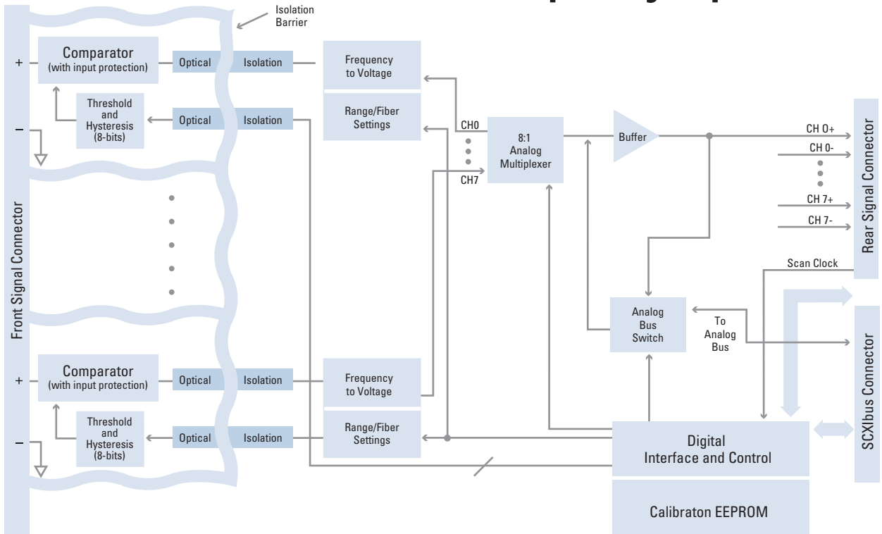
Figure 1. SCXI-1126 Block Diagram
