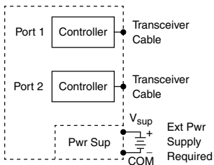
Figure 1. sbRIO-9860 Hardware Overview
