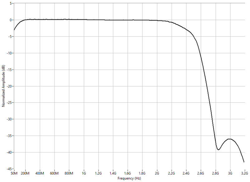
Figure 12. Analog Output Single Channel Mode Frequency Response With Anti-Image Filter, Measured 19
