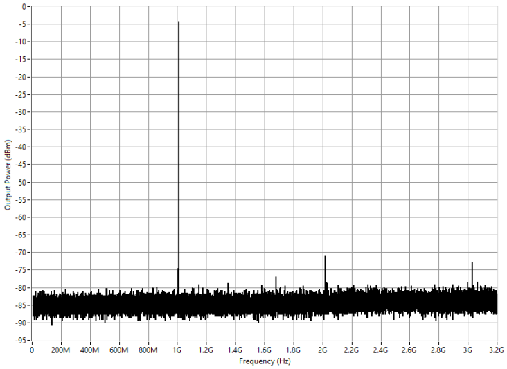
Figure 9. Single Tone Spectrum (Single Channel Mode, 1.01 GHz 0 dBFS), Measured 16
