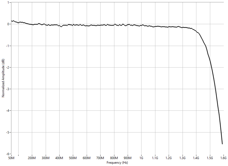
Figure 10. Analog Output Dual Channel Mode Frequency Response, Measured 18
