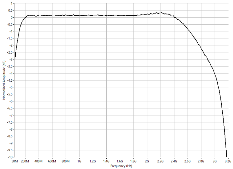
Figure 11. Analog Output Single Channel Mode Frequency Response, No Anti-Image Filter, Measured 18
