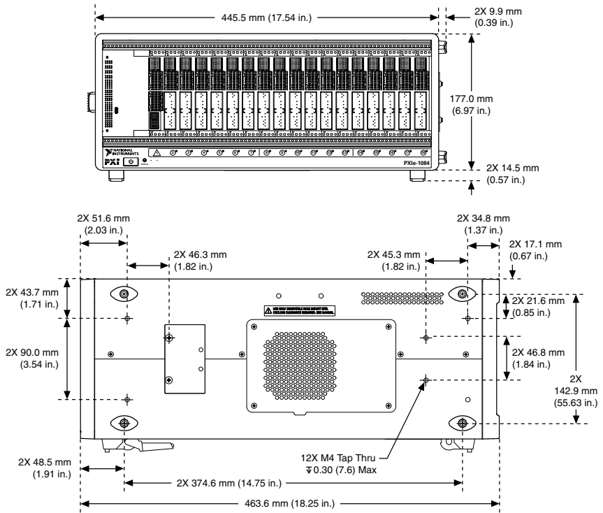
Figure 1. PXIe-1084 Chassis Dimensions (Front and Side)
