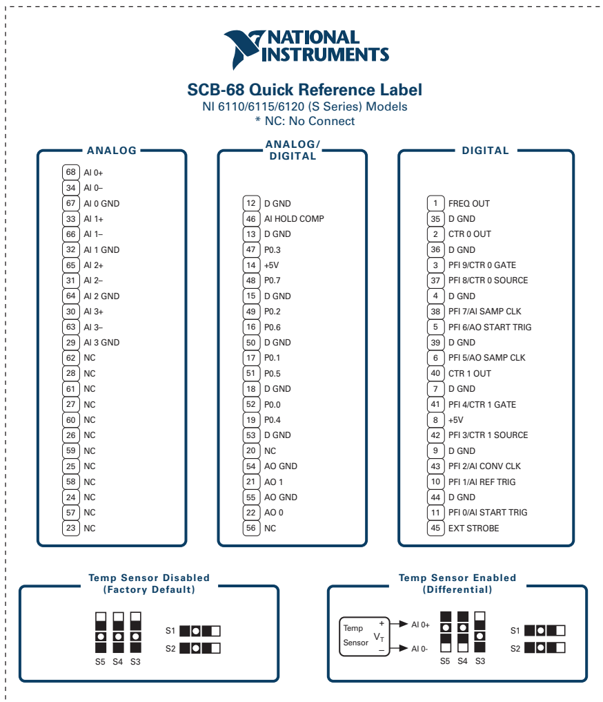
Figure 1. NI 6110/6115/6120
