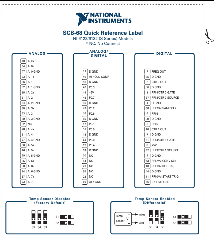
Figure 4. NI 6123/6133/6143
