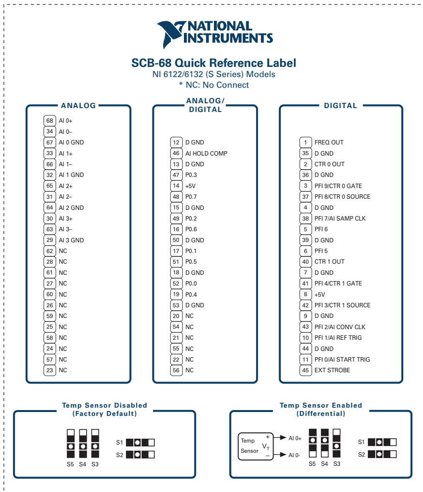
Figure 3. NI 6122/6132
