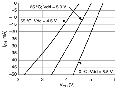
Figure 1. P0.<0..1>: I_{OH} versus V_{OH}
