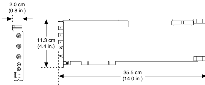
Figure 6. PCI-5153 Dimensions
