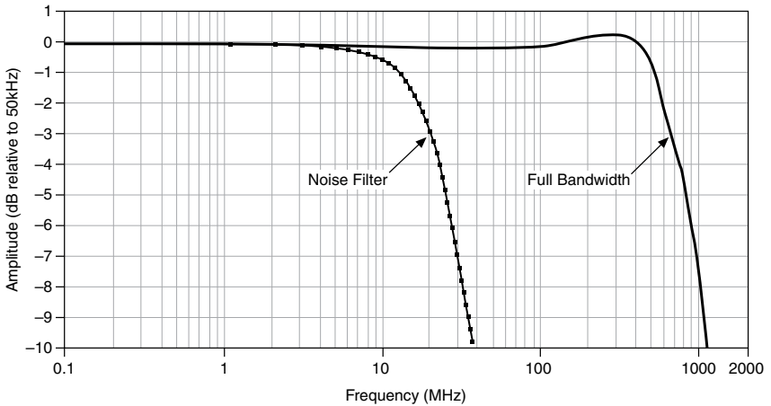
Figure 1. PCI-5153 Frequency Response, 5 V pk-pk through 0.1 V pk-pk Input Ranges (Measured)
