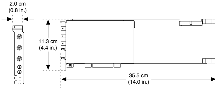
Figure 6. PCI-5153 Dimensions
