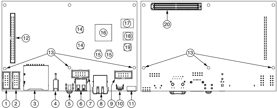
Figure 2. sbRIO-9627 Components
