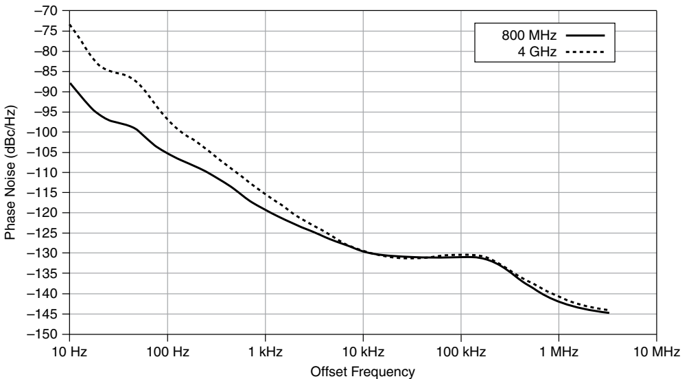
Figure 1. PXIe-5667 (7 GHz) Phase Noise at 800 MHz and 4 GHz Center Frequency (Nominal)
