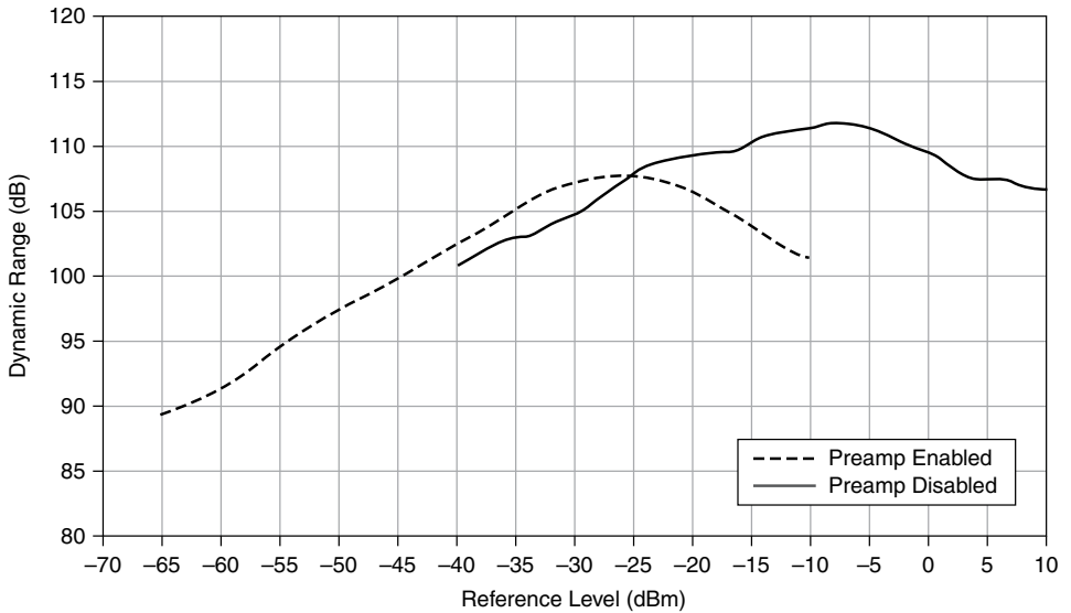
Figure 6. Dynamic Range versus Reference Level (Nominal) 43
