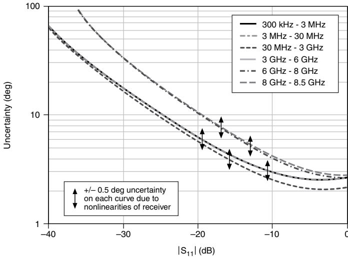
Figure 10. PXIe-5632 Phase Uncertainty (Typical)
