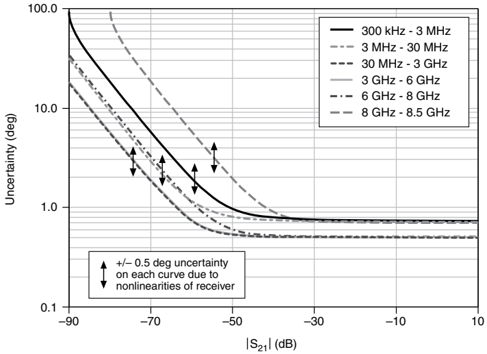
Figure 8. PXIe-5632 Phase Uncertainty (Typical)
