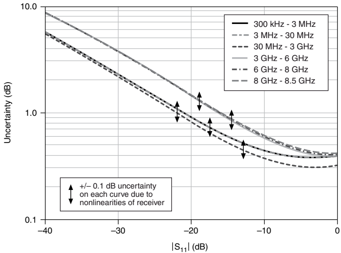
Figure 9. PXIe-5632 Magnitude Uncertainty (Typical)
