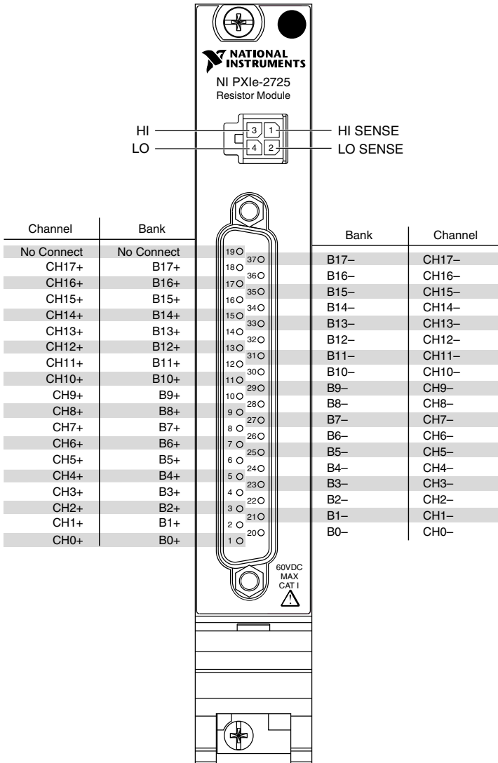
Figure 3. NI 2725 Connector Pinout
