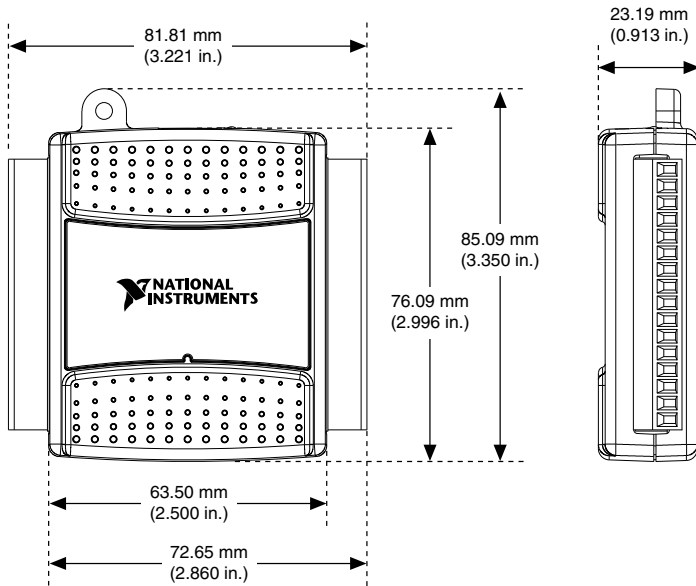
Figure 1. USB-6009 Dimensions
