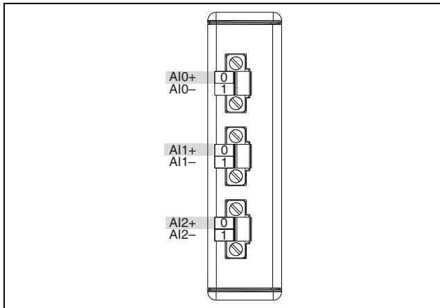
Figure 2. NI 9225 Terminal Assignments
