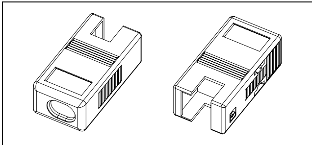
Figure 1. NI 9971 Connector Backshell
