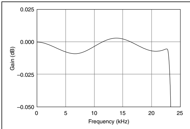
Figure 7. Typical Passband Response of the NI 9225
