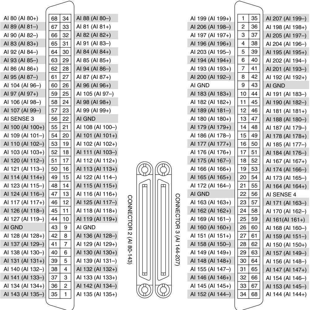
Figure 8. NI PXIe-6375 Connectors 2 and 3 Pinout
